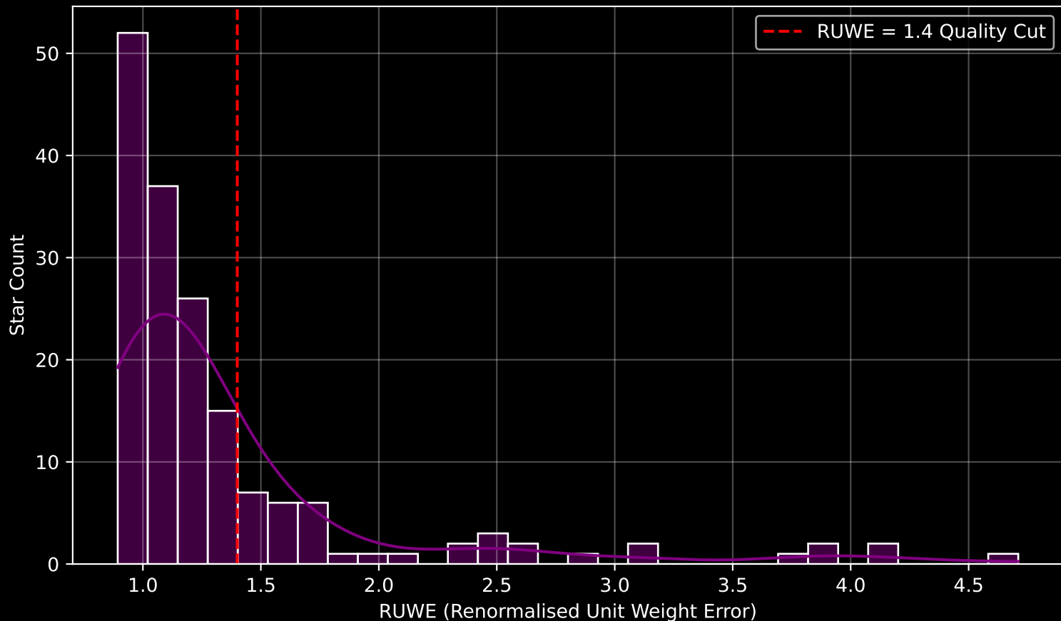
GAPOGEE DR17 Field [145+62_MGA] RUWE Distribution (n= 168)
