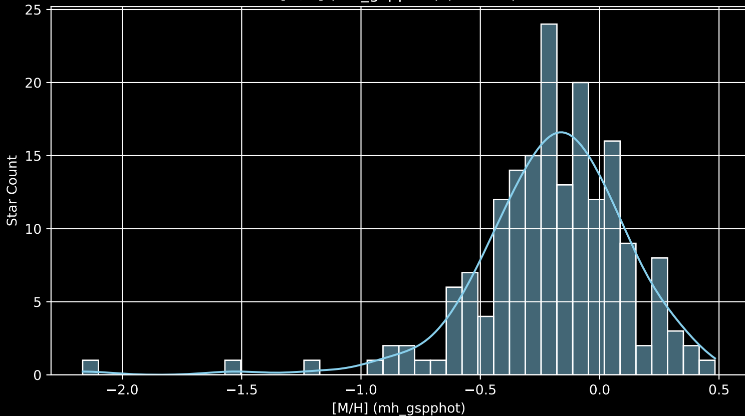
APOGEE DR17 Field: [145+62_MGA [M/H] (mh_gspphot) (n= 178)
