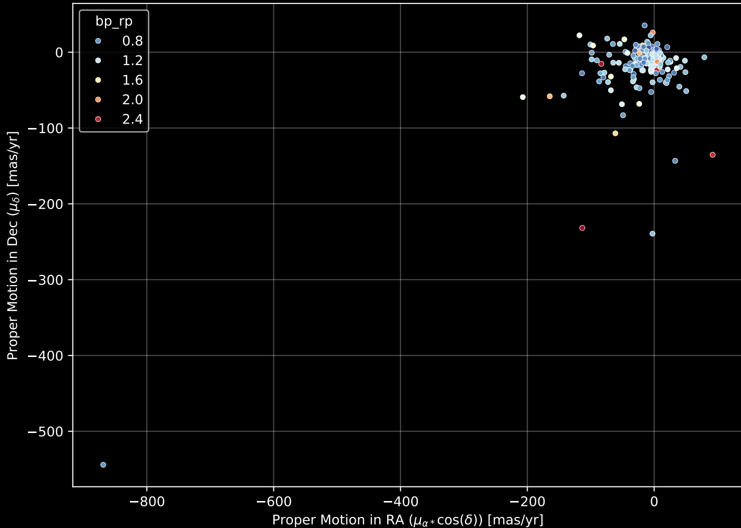
APOGEE DR17 Field: [145+62_MGA] Proper Motion Diagram (n= 181)
