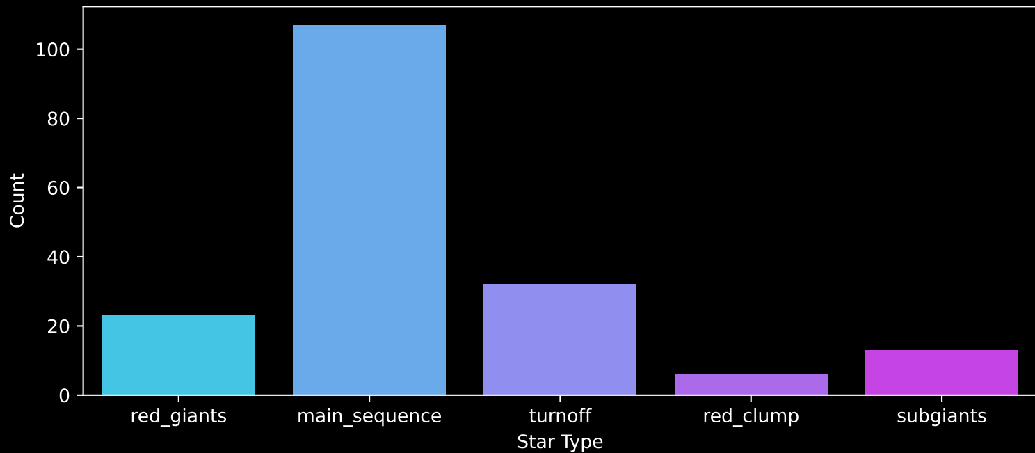
APOGEE DR17 Field: [145+62_MGA] Count plot of Star Type
