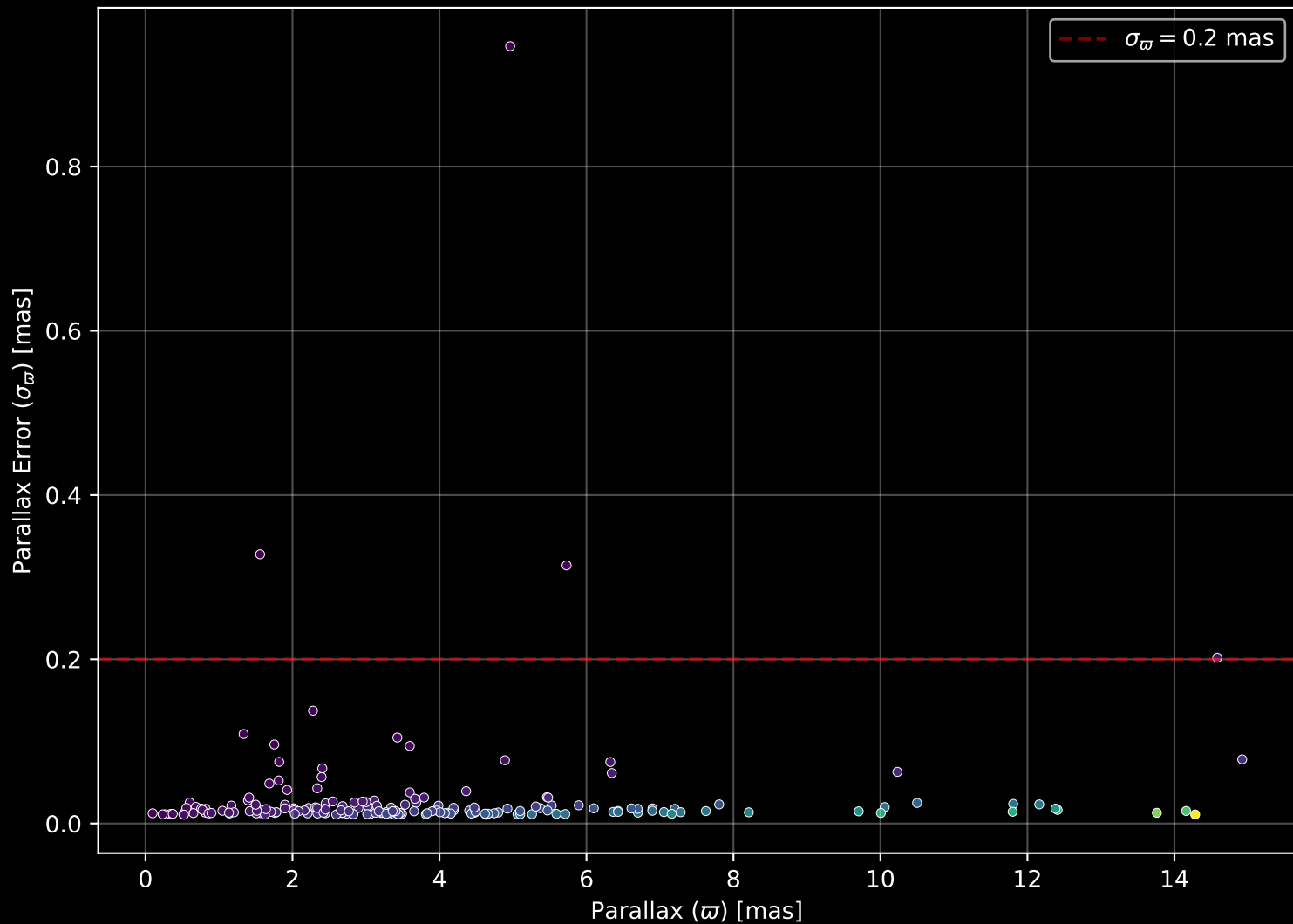
APOGEE DR17 Field: [145+62_MGA] Parallax Quality (n= 181)
